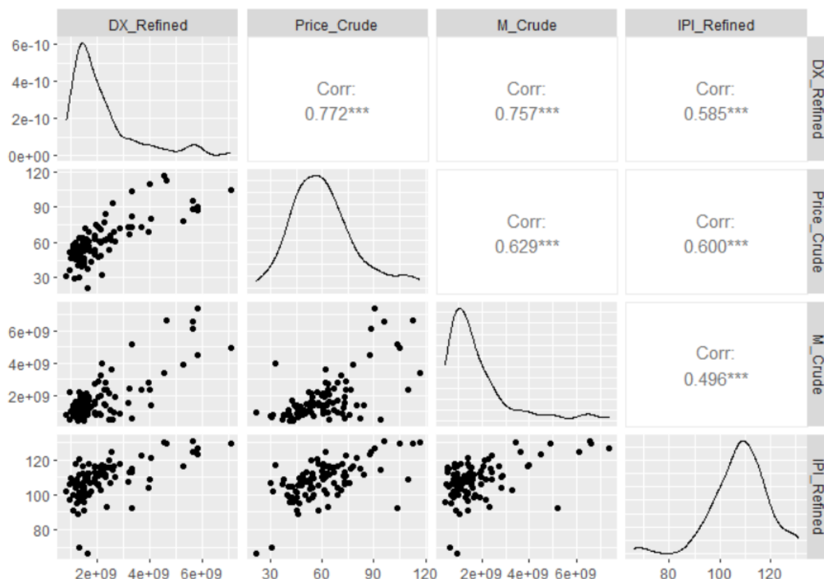
Exhibit ii: Pearson's Correlation and Scatter Plots Matrix
