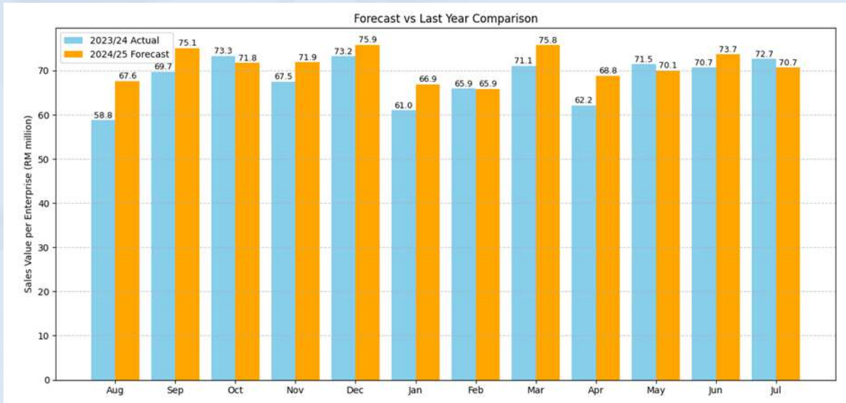
Graph 2(f) : Comparison of Sales Forecast Value and Actual Sales Value (YoY)
