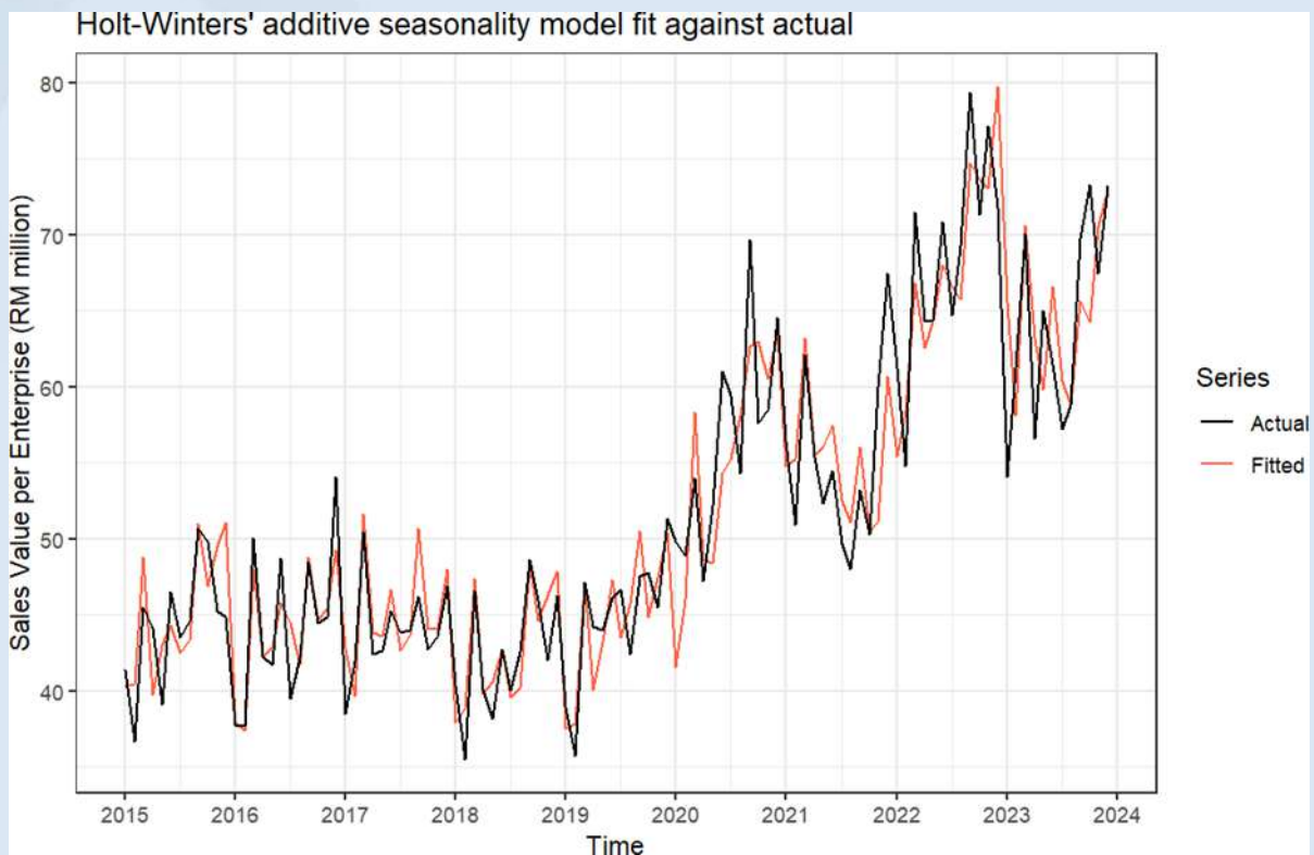
Graph 2(d) : Holt-Winters' Additive Seasonality Model Fit Against Actual
