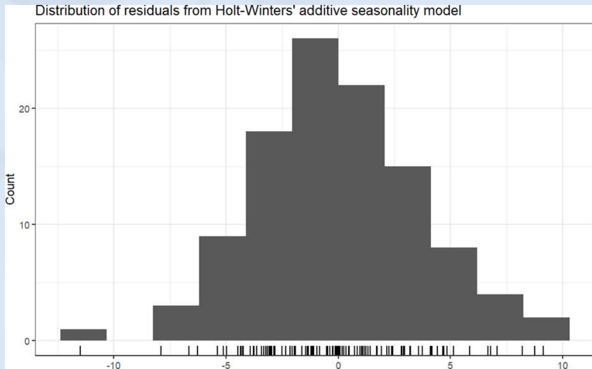
Graph 2(i) : Distribution of Residuals from Holt-Winters' Additive Seasonality Model
