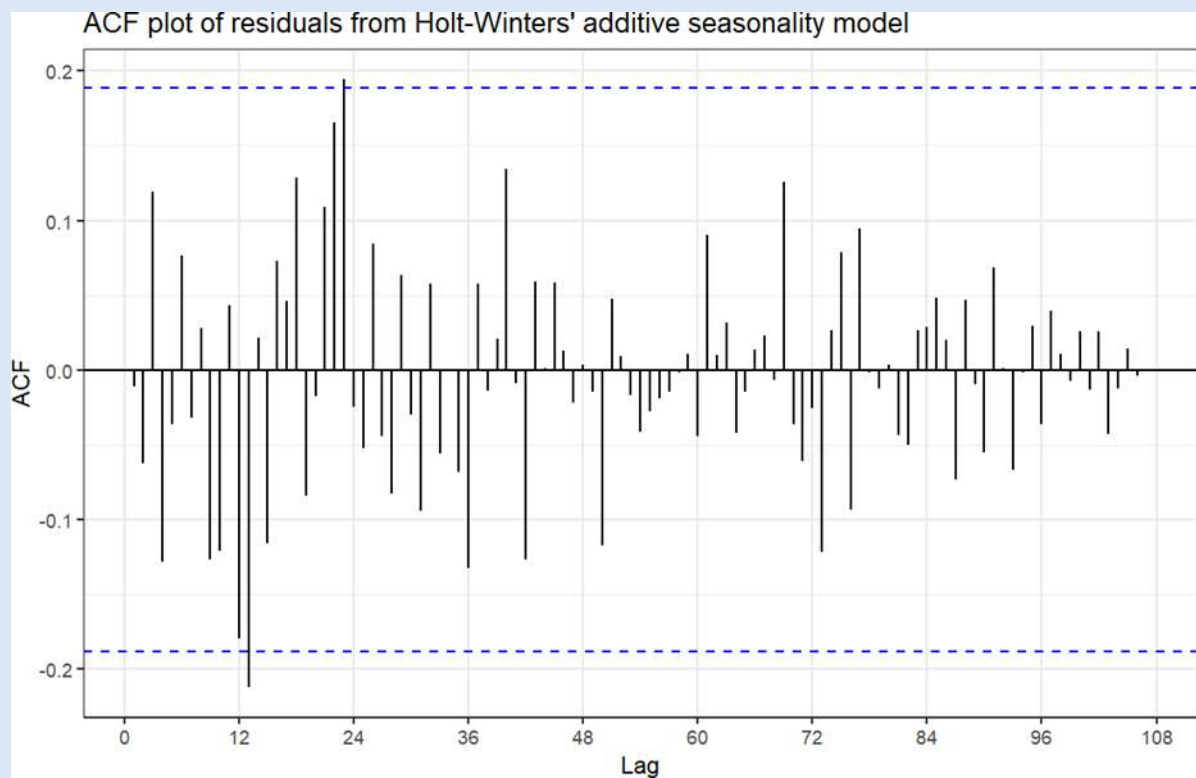
Graph 2(h):ACF Plot of Residuals from Holt-Winters' Additive Seasonality Model
