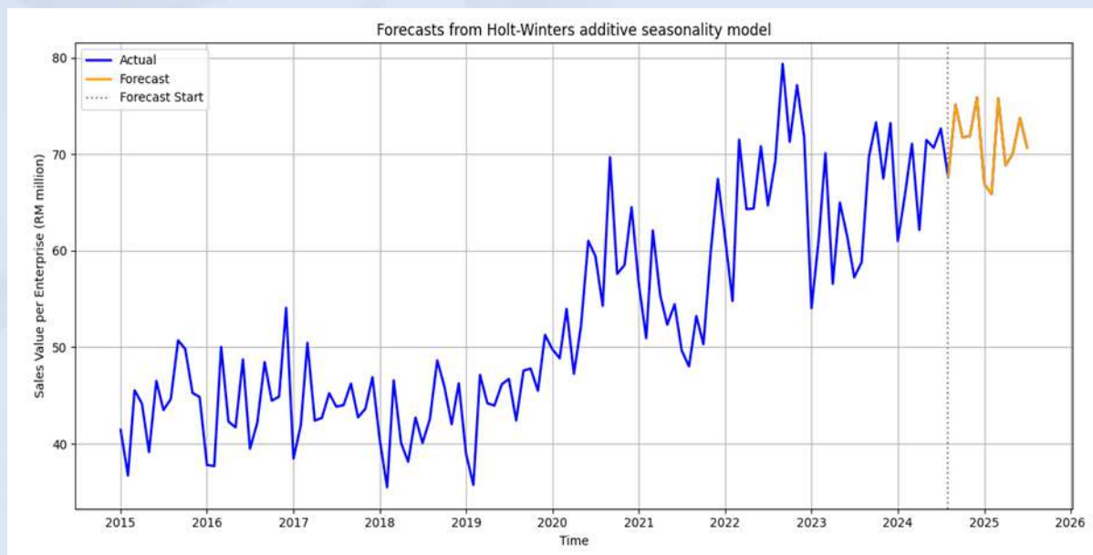
Graph 2(e) : Forecasts from Holt-Winters' Additive Seasonality Model
